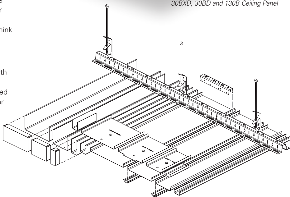
30BXD, 30BD and 130B Ceiling Panel
